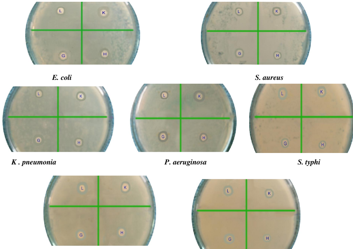
FIGURE 1. Anti bacterial activities of kidney, liver, heart and gill proteins of Labeo rohita against different clinical isolates
