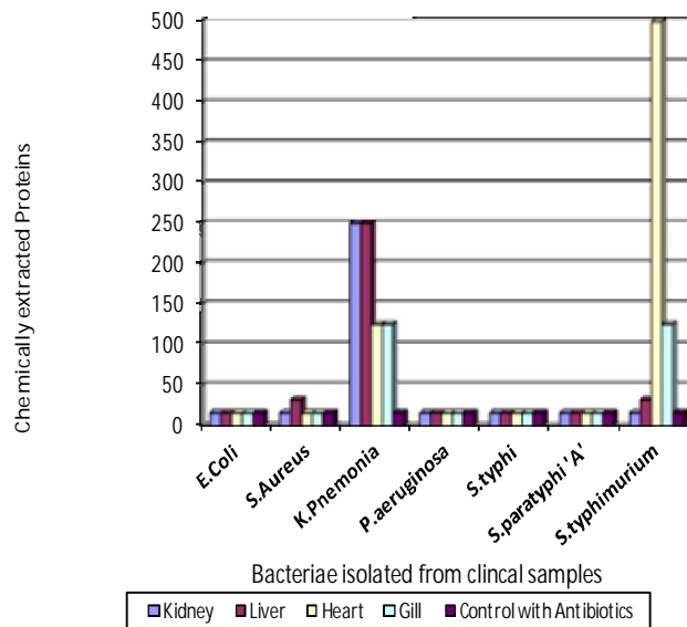
FIGURE 2. Minimum Inhibitory Concentrations of different tissue proteins of Labeo rohita against different clinical isolates
