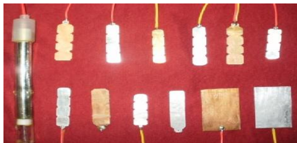
Figure (1): Electrodes and cells of different size & shape
